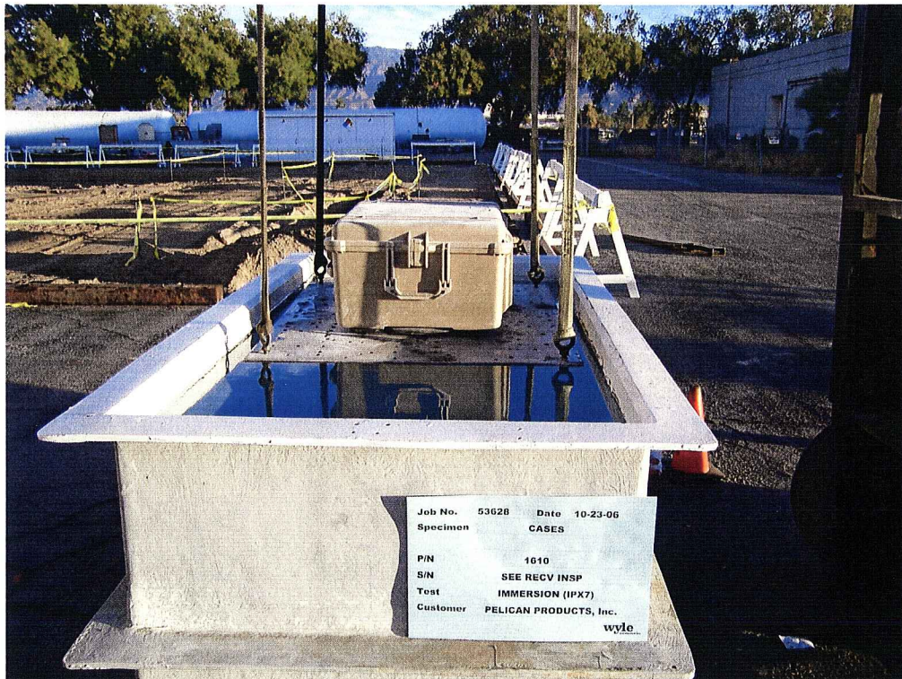
Photograph 8 Immersion Test Setup
