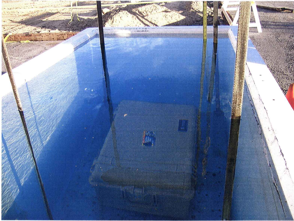
Photograph 9 Immersion Test Setup
